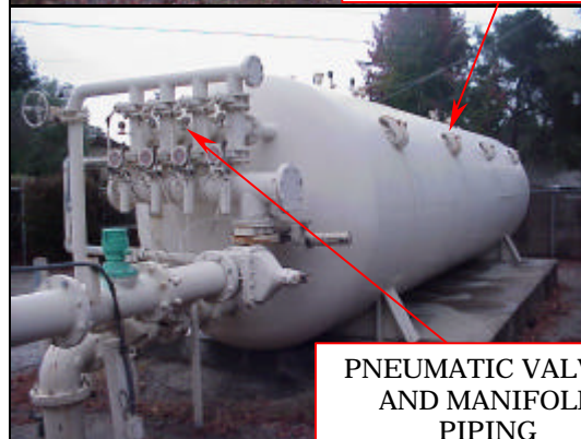
FILTER VESSEL ACCESS HATCH (4)
